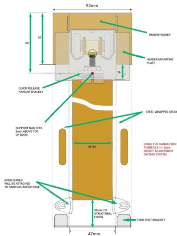
Section Showing Timber Door Installation
